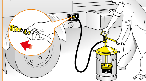
Filling central greasing system
